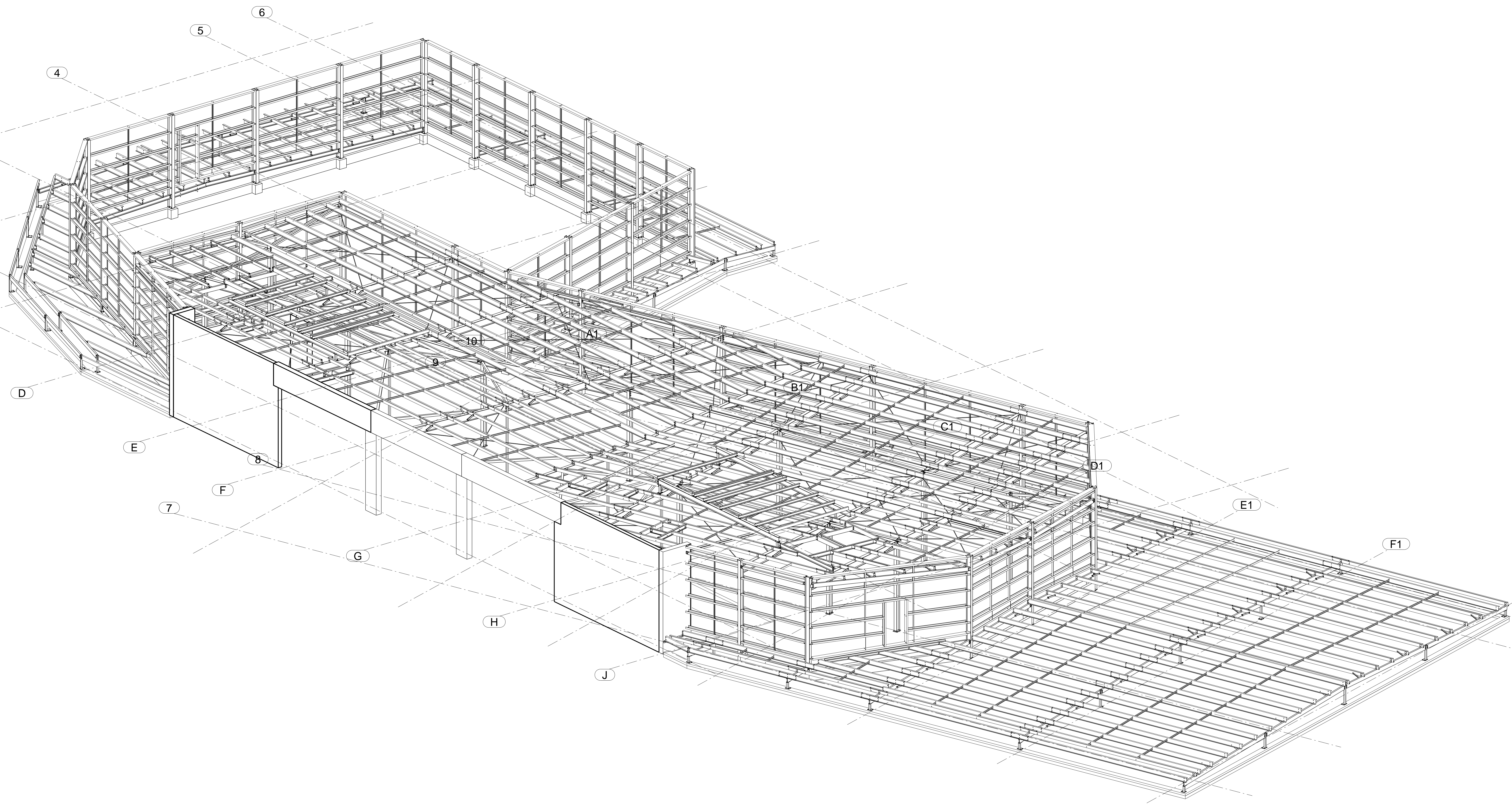
ISOMETRIC VIEW
